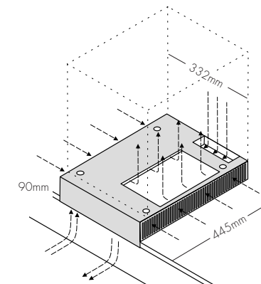
Simple-fit Ventilation Base A refined and simple-to-install ventilation kit is included with the S2 system.
